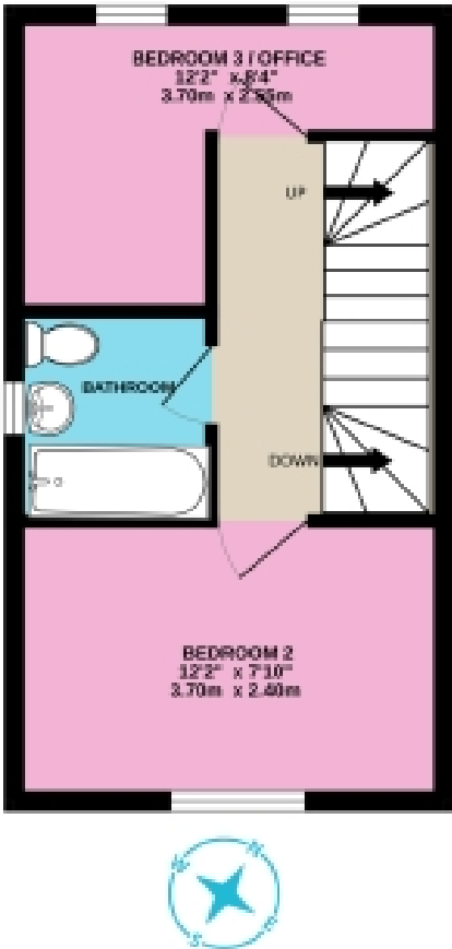
3-BEDROOM END TERRACE HOUSE
